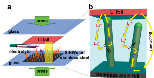
Figure 1. Schematic diagrams showing (a) the prelithiation of SiNWs on stainless steel (SS) foil, and (b) the internal electron and \text{Li}^+ pathways during the prelithiation. Two possible electron pathways are shown in (b). Electron can directly flow into the SiNW if the nanowire tip contacts the Li foil, or the electron can flow across the contacting point of Li foil and SS and enter the SiNW through the bottom.
