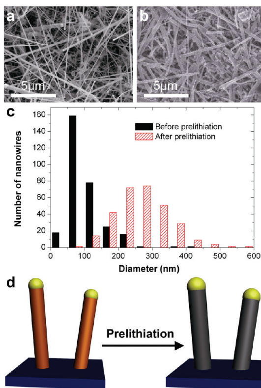
Figure 2. SEM images of SiNWs (a) before and (b) after 10 min prelithiation. After prelithiation, the SiNWs were washed with acetonitrile before taking SEM images. (c) Size distribution of SiNWs before and after prelithiation. (d) Schematic showing the increase of SiNW diameter after prelithiation.
